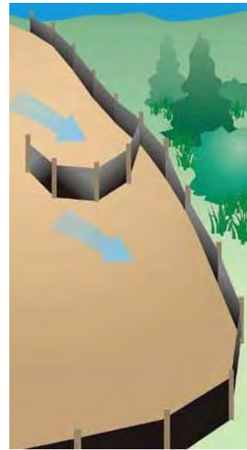
“J-hooked” silt fencing
